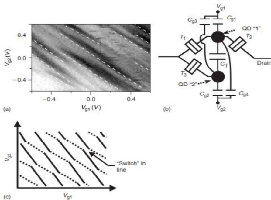
Fig. 1 In a Nc-Si Point-contact, electrostatic coupling has an impact. ( a ) A dim scale plot of the current as a function of two door voltages at 4.2 K. Vds 2 mV and the most outrageous worth of Ids 1 nA (white). ( b ) the twofold quantum speck model c) schematic of Coulomb faltering lines [18].
