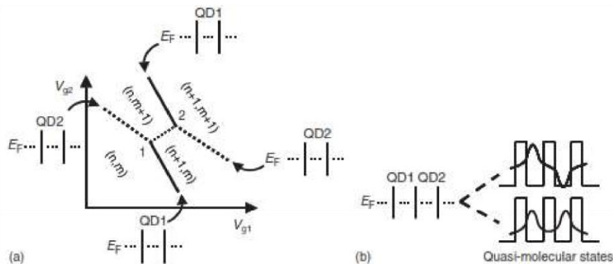
Fig. 2 Electron Wavefunction Coupling Effects in a Nc-Si Point-Contact. (a) Resonance (at points “1” and “2”) between energy levels on two quantum dots, in a plot of the Coulomb oscillations versus the gate voltages V_{g1} and V_{g2} . (b) Quasi-molecular states [11].
